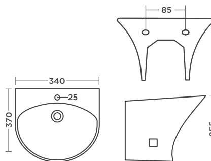
Integrated Wall Hung Basin L340 W370 H255mm
