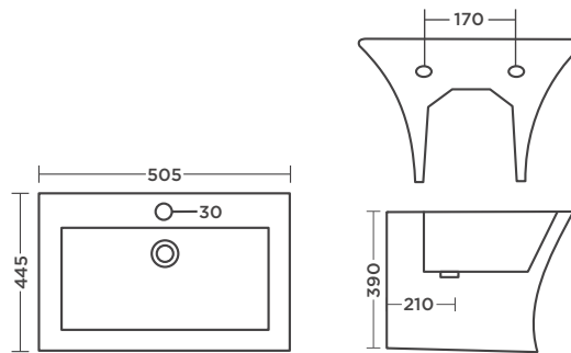
Integrated Wall Hung Basin L505 W445 H390mm
