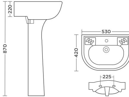
Full Pedestal Basin L530 W420 H870mm
